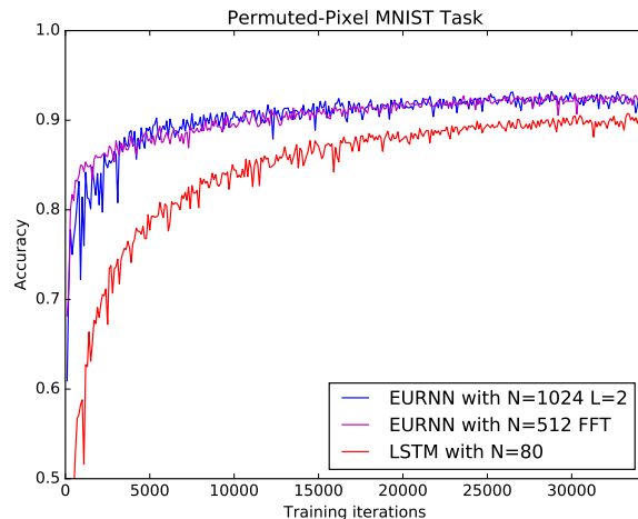
Figure 3. Pixel-permuted MNIST performance on the validation dataset.
