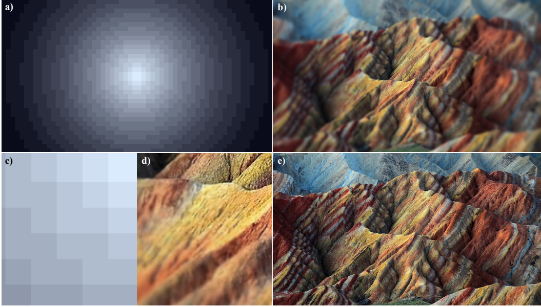
Figure 1: a) : A 1920 \times 1080 (PNG) image divided into 32 \times 32 pixel blocks, each colored according to its distance from the fixation point (image center). b) : Foveated 1920 \times 1080 image, computed with our foveated optimization scheme based on adaptive gaussian blurring (generated at a rate of 165 Hz) c) : Close up of image a ) at transition from fovea into periphery. d) : Corresponding close up of image b ). e) : Original image. Notice that even without image blending such as cosine windowing functions, the final foveated output from b ) looks smoothly generated in reference to e ).
