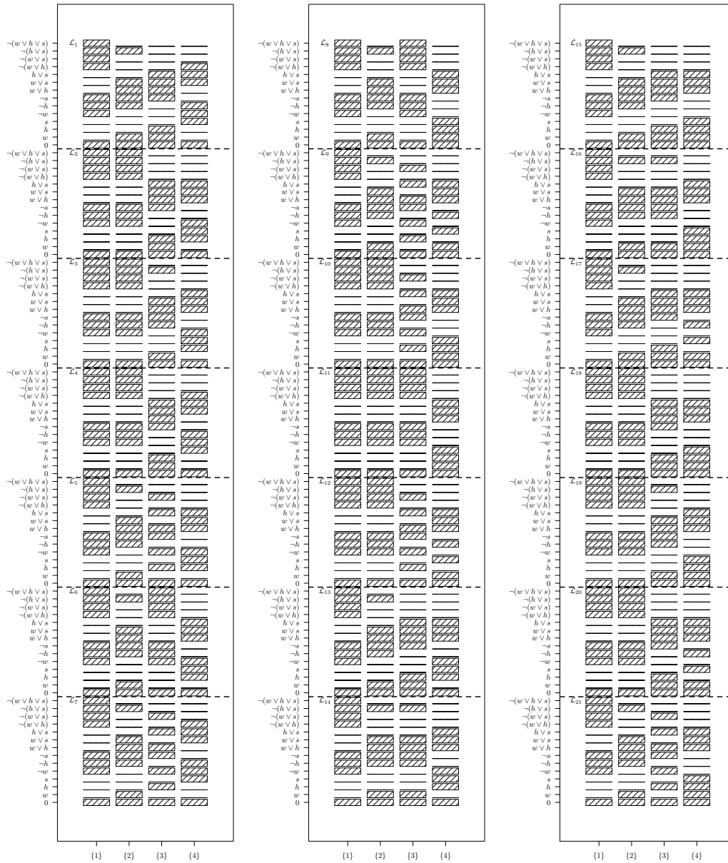
Figure 13: The 21 refined lexica for formalization of Example (11) in Section 5.7.
