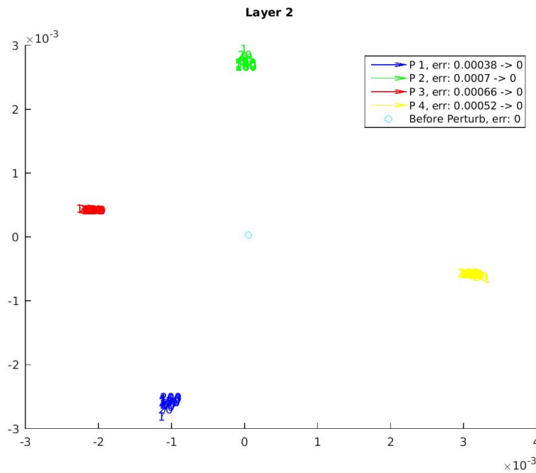
Figure 32: Multidimensional scaling of the layer 2 weights throughout the retraining process. There are 4 runs indicated by 4 colors/trajectories, corresponding exactly to Figure 41. Each run corresponds to one perturbation of the model M_{final} and subsequent 200 epochs' training. The number in the figure indicates the training epoch number after the initial perturbation.
