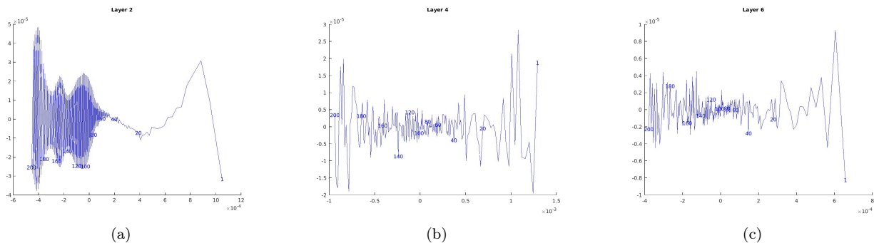
Figure 22: The Multidimensional Scaling (MDS) of the layer 2/4/6 weights of model M_5 throughout the retraining process. Only the weights of one run (run 1 in Figure 41) are fed into MDS to provide more resolution. The number in the figure indicates the training epoch number after the initial perturbation.
