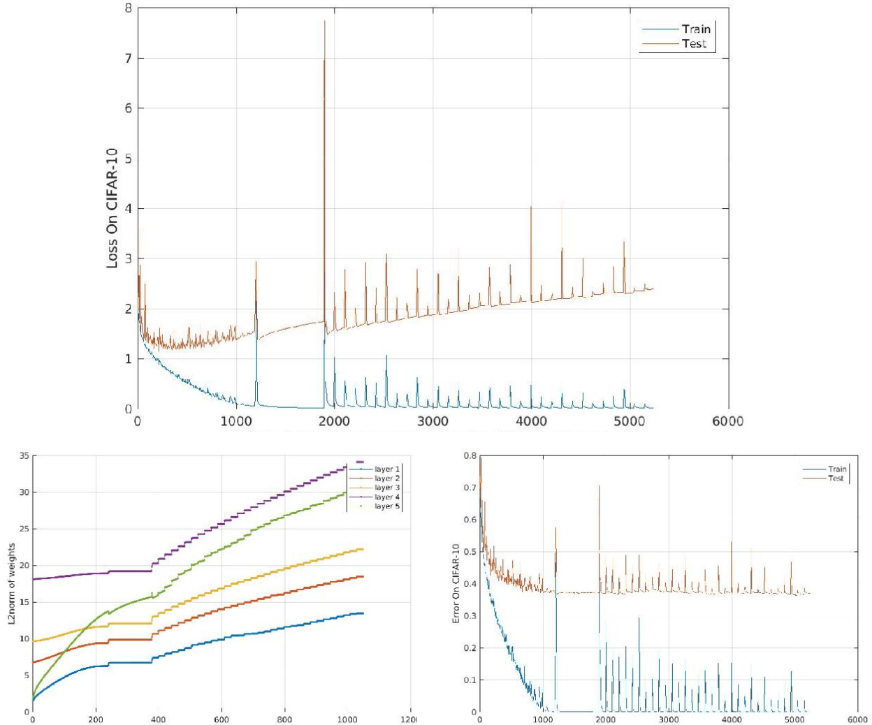
Figure 3: We train a 5-layer convolutional neural networks on CIFAR-10 with Gradient Descent (GD) on crossentropy loss. The top plot shows the crossentropy risk on CIFAR during perturbations (see text). The bottom left is the corresponding square norm of the weights; the bottom right plot shows the classification error (see text). The network has 4 convolutional layers (filter size 33, stride 2) and a fully-connected layer. The number of feature maps (i.e., channels) in hidden layers are 16, 32, 64 and 128 respectively. Neither data augmentation nor regularization is performed. Initially, the network was trained with GD as normal. After it reaches 0 training classification error (after roughly 1800 epochs of GD), a perturbation is applied to the weights of every layer of the network. This perturbation is a Gaussian noise with standard deviation being \frac{1}{4} of that of the weights of the corresponding layer. From this point, random Gaussian noises with the such standard deviations are added to every layer after every 100 training epochs. The empirical risk goes back to the original level after added perturbations, but the expected risk grows increasingly higher. As expected, the L_2 -norm of the weights increases after each step of perturbation followed by gradient descent which resets the empirical risk to zero. Compare with Figure 14 and see text.
