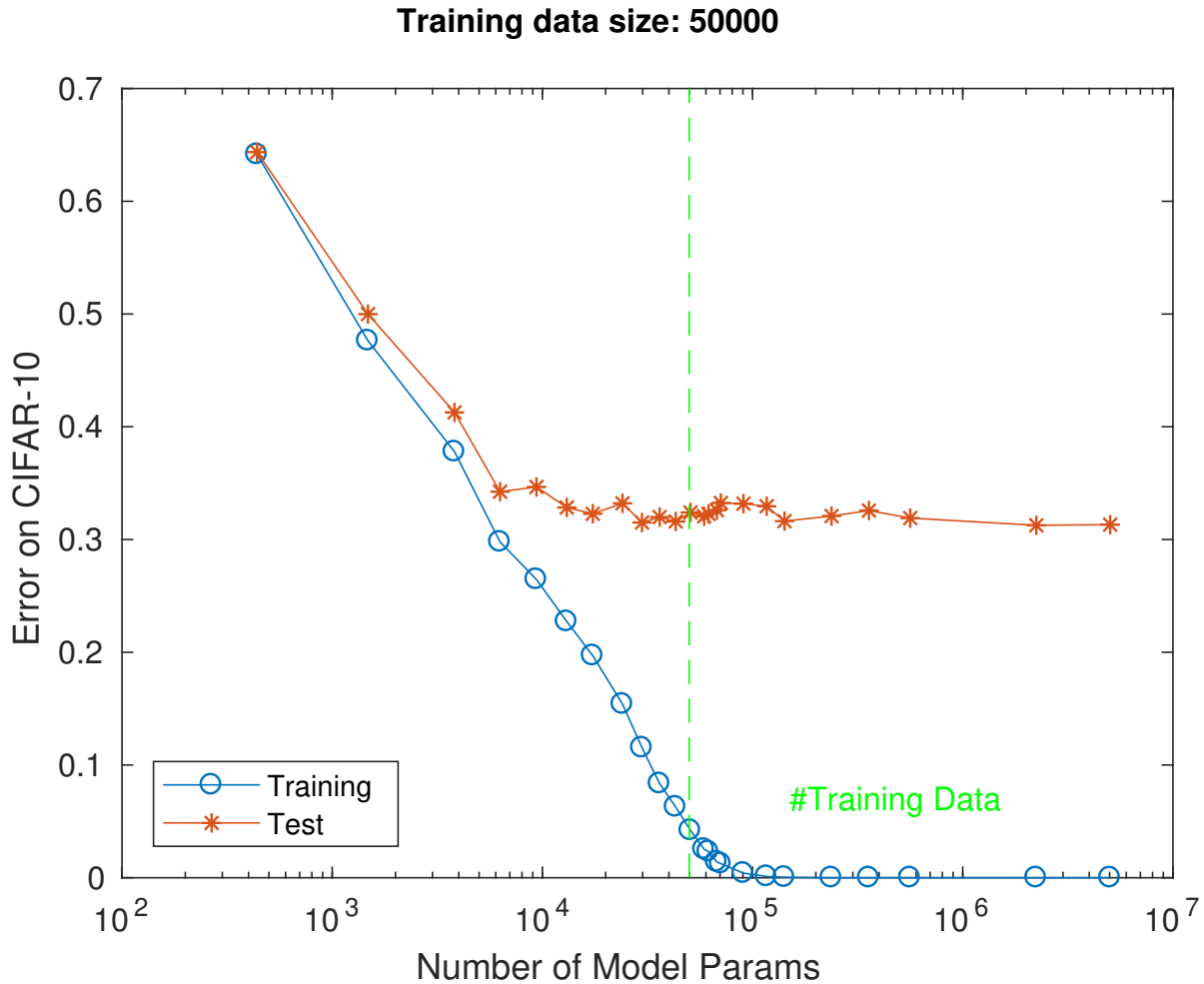
Figure 6: The figure shows the classification error under the same conditions of Figure 5. The classical theory explains the generalization behavior on the left; the text explains the lack of overfitting for W > N .
