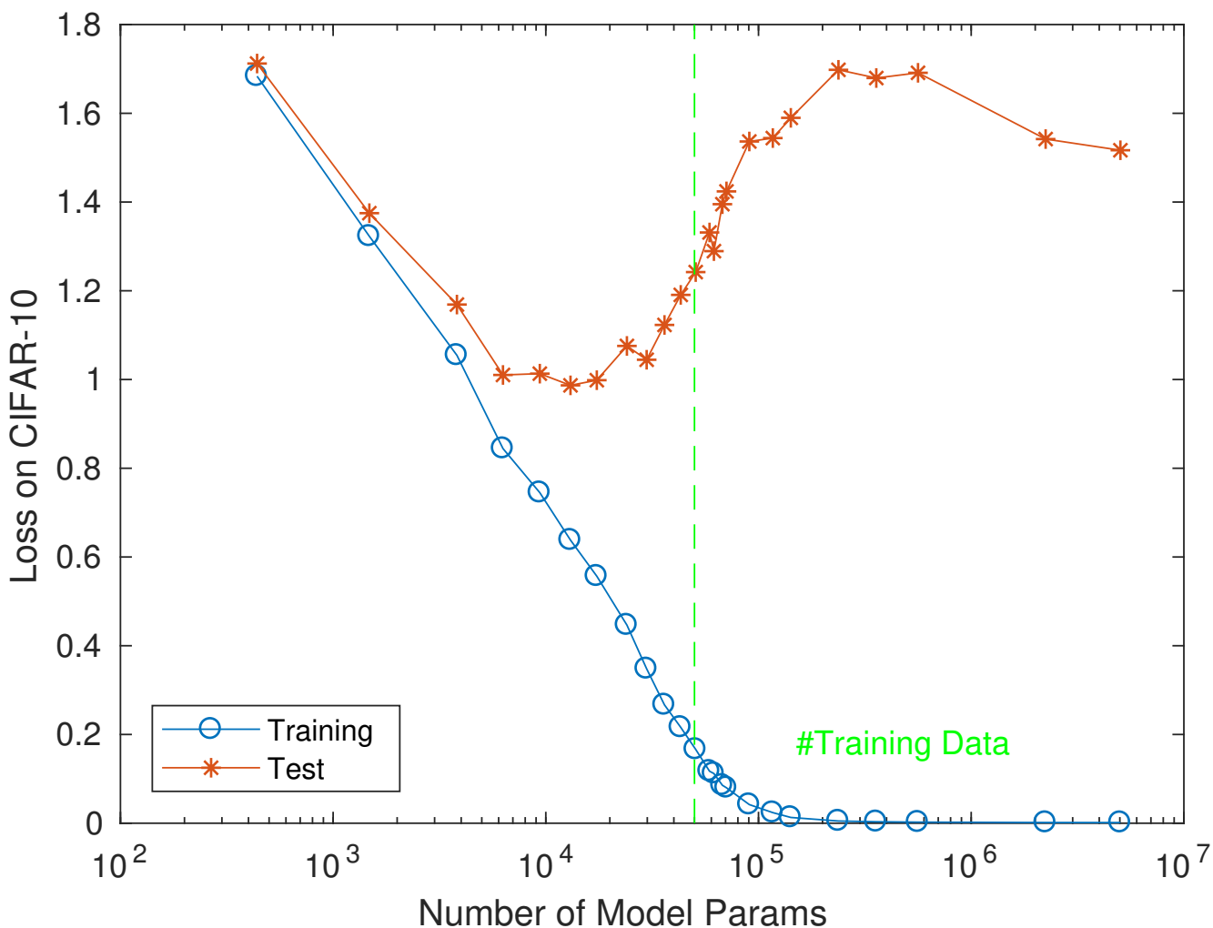
Figure 5: The previous figures show dependence on n – number of training examples – for a fixed ReLU architecture with W parameters. This figure shows dependence on W of the cross entropy risk for a fixed training set of n examples. The network is again a 5-layer all convolutional network (i.e., no pooling) with ReLUs. All hidden layers have the same number of channels. Neither data augmentation nor regularization is performed. SGD was used with batch size = 100 for 70 epochs for each point. There is clear overfitting in the expected risk.
