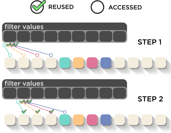
Figure 12: Data reuse through local variables improves performance of the kernel. The convolution operation has a great deal of overlap at neighboring pixels. A thread is able to store values in registers and perform four pixels worth of convolution, allowing a single access of constant or shared memory to serve multiple convolution operations. Step 1 shows reuse of the first filter value. In Step 2, the second filter value is likewise reused but so are three of the four image pixels previously accessed.
