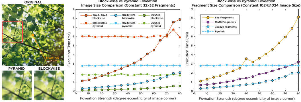
Figure 5: Evaluation is performed with RGB 8-bit images on a GTX 1060 GPU. For the block-wise approach, CUDA kernel execution is timed. For the Pyramid approach, mipmap generation and sampling is timed (See Appendix 5.1). Note that blue lines represent the same data in both figures.
