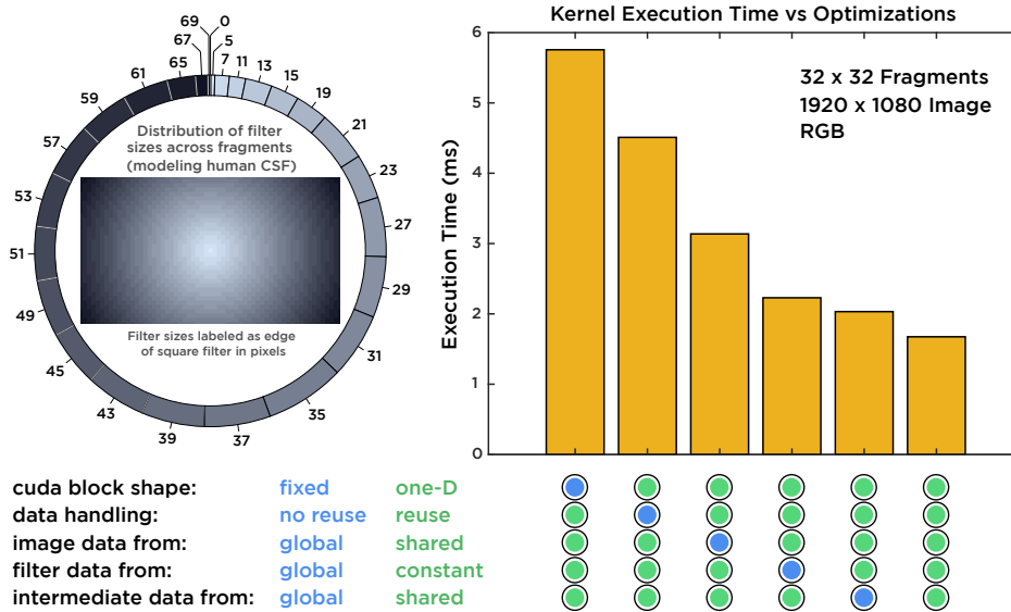
Figure 10: Impact of optimizations on performance. Evaluation done on NVIDIA GTX 1060 GPU (6 GB). Only kernel execution times are shown - memory transfers excluded.
