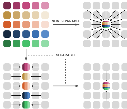
Figure 7: Separable convolution is faster than non-separable convolution. Although the separable approach requires more operations to produce a single output pixel, the intermediate horizontal result is re-used for the vertical step by several pixels, leading to a net decrease in the number of operations.
