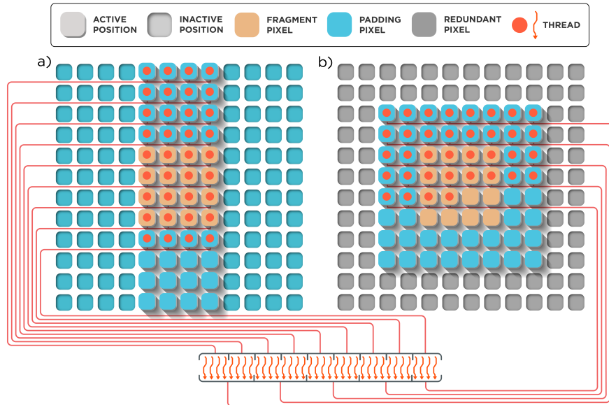
Figure 11: A one-dimensional block of threads can be optimally arranged for any purpose. a) Threads arranged in a vertical column for horizontal convolution. b) Threads arranged to transfer a small tile of image data into shared memory.
