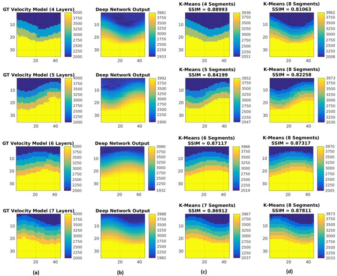
Figure 7. Tomography with 4-7 velocities: (column a) Ground truth (column b) DNN output image (column c) Segmented image using K-Means and the correct number of layers; and (column d) Segmented image using K-Means and 8 layers.
