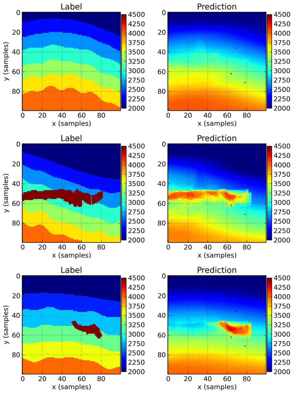
Figure 8. In the top row left column a layered model is presented as ground truth (label), the right column shows the prediction generated with the trained model. That model was training with data that only contains layered models with different number of layers and velocity per layer. The predicted model closely resembles the
