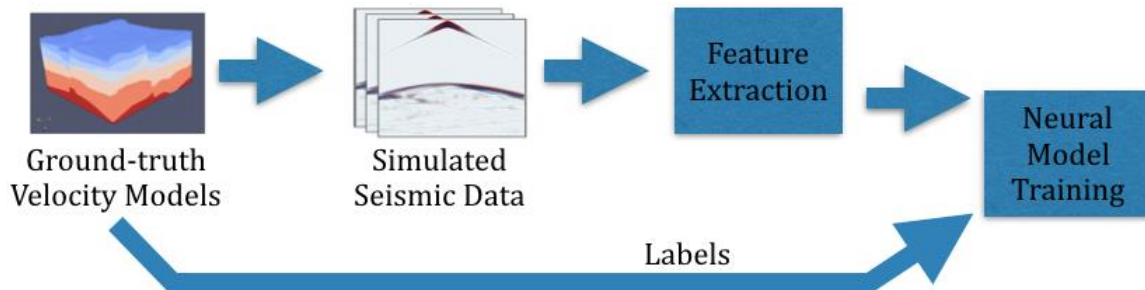
Figure 3. Training workflow.
