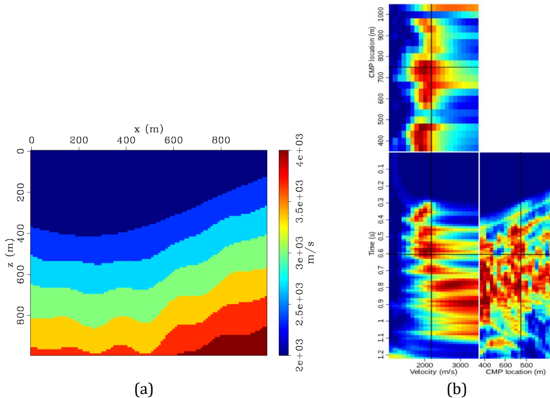
Figure 6. An example of a calculated semblance cube for a seven-layer model. Note that the traditional velocity analysis panel of the semblance cube shown in (b) captures each of the layer interfaces. Also, note that the right panel (axes of CMP location and zero-offset time) of the semblance cube qualitatively gives the approximate structure of the velocity model shown in (a).
