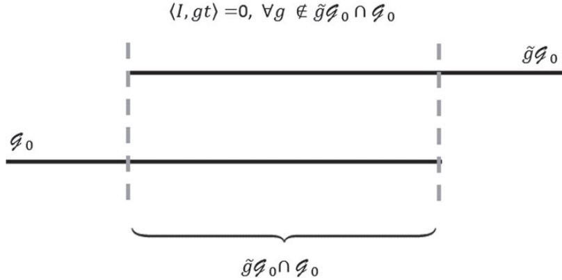
FIG. 1. A sufficient condition for invariance for locally compact groups: if \langle gI, t \rangle = 0 for all g \in \tilde{\mathcal{G}}_0 \Delta \mathcal{G}_0 , the integral of \eta_b \langle I, gt \rangle over \mathcal{G}_0 or \tilde{\mathcal{G}}_0 will be equal.
